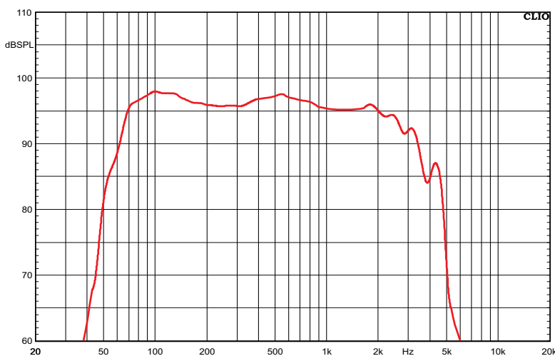
Woofer inside recommended cabinet (60 liters tuned at 55Hz), 2PI
